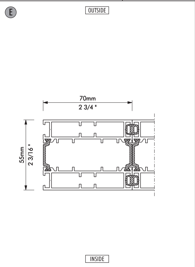
Description: Horizontal-Section, frame extension 70 mm System: SF55 Detail-No.: SF55-110
