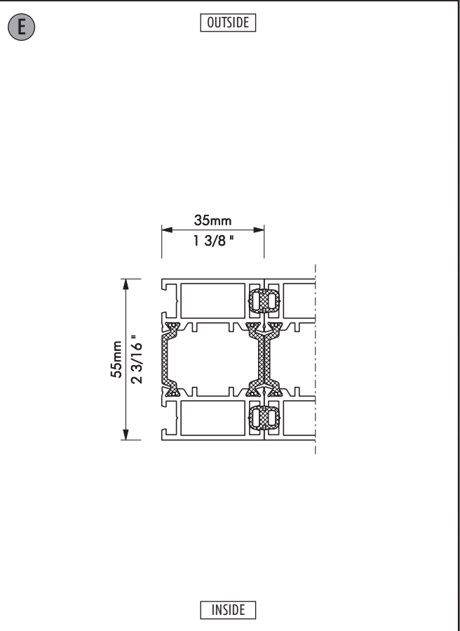
Description: Horizontal-Section, frame extension 35 mm System: SF55 Detail-No.: SF55-109
