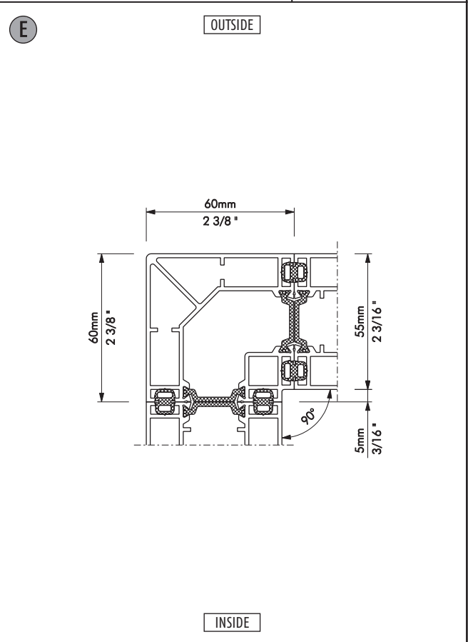
Description: Horizontal-Section, 90°- connection profile System: SF55 Detail-No.: SF55-111
