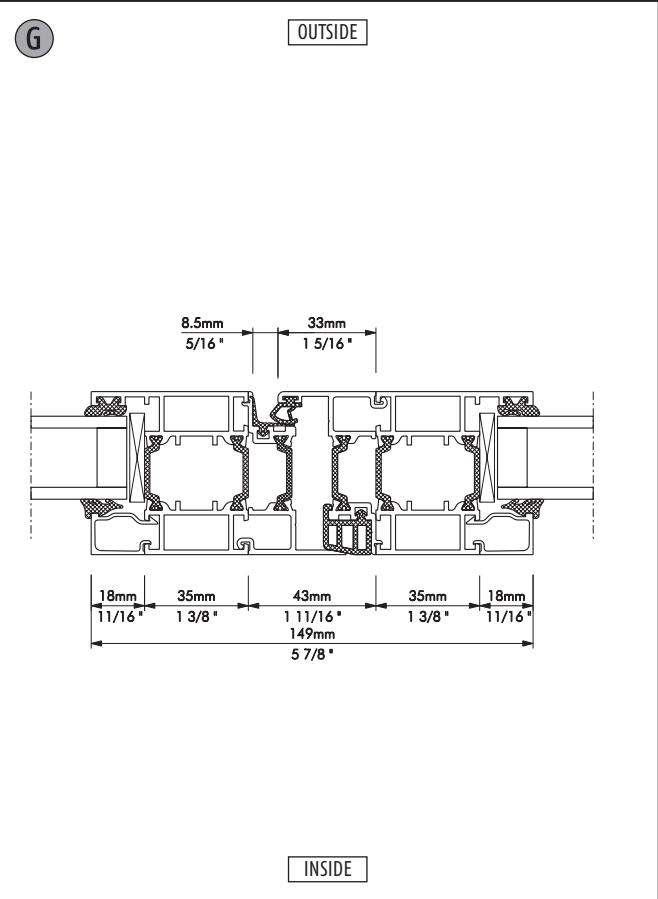
Description: Horizontal-Section, panel - panel closing section System: SF55 Detail-No.: SF55-108
